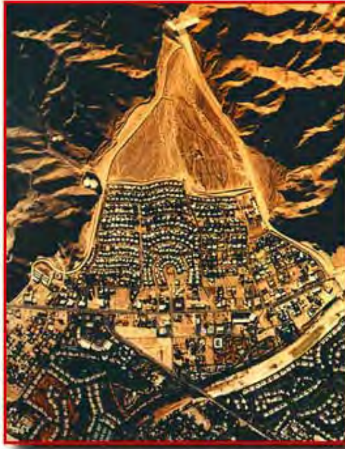
Figure 1-8. An alluvial fan can have numerous channels.
